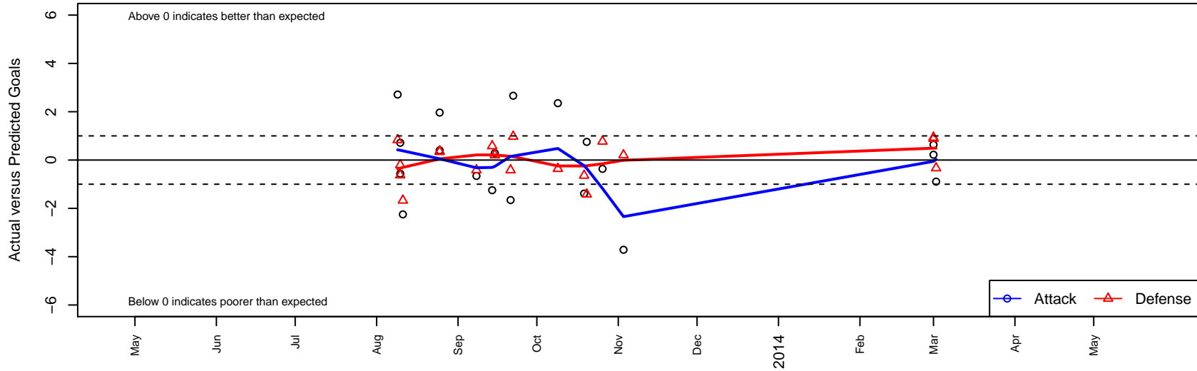
SoccerEdge Academy Black G00 Dots are actual minus expected GF (blue circles) and GA (red triangles). Blue line is smoothed change in attack strength. Red is smoothed change in defense strength.
